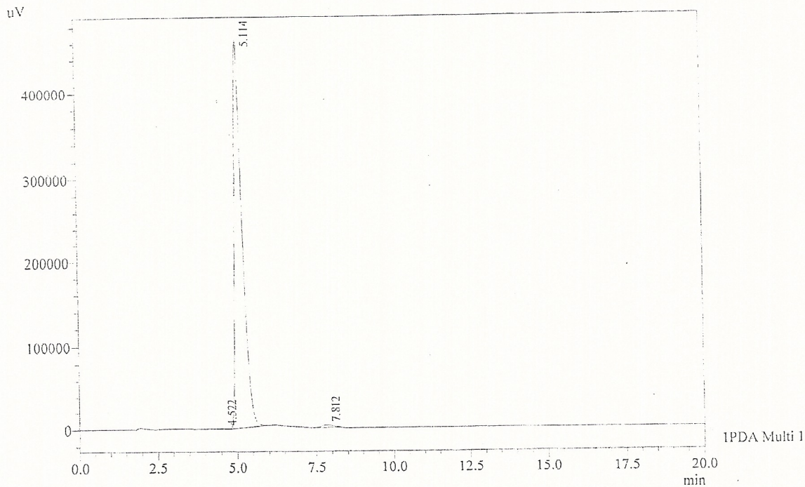
Chromatogram Coumestrol D:\promonence\Data\2013\JAN-2013\250113F.lcd
